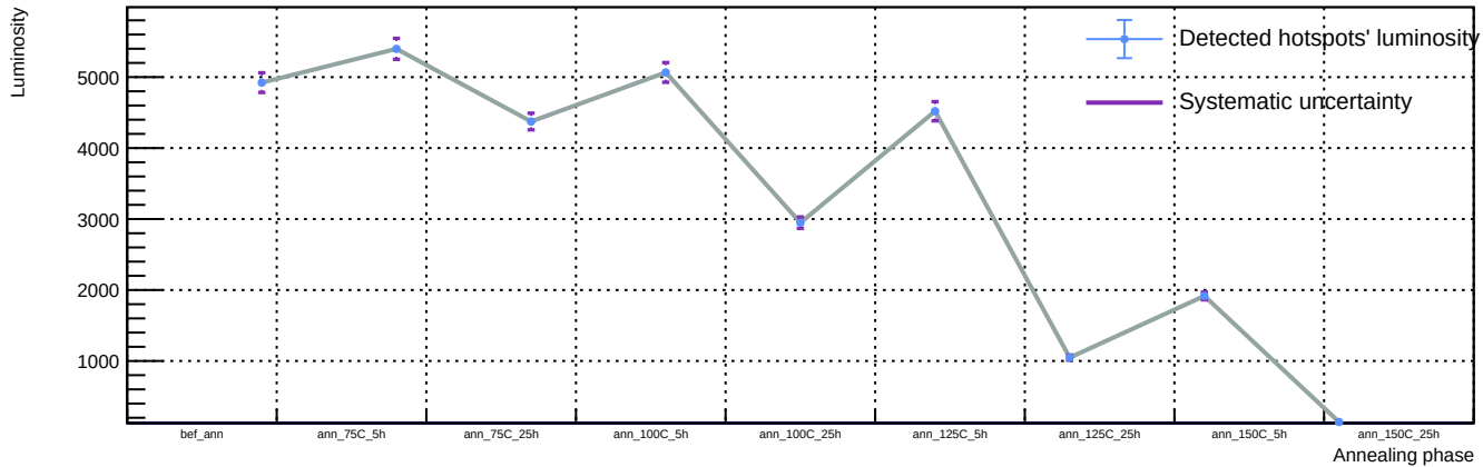
Sensor A1, T = 20\text{ C} , v_{\text{over}} = 7\text{ V} - Spot 77: luminosity vs phase
