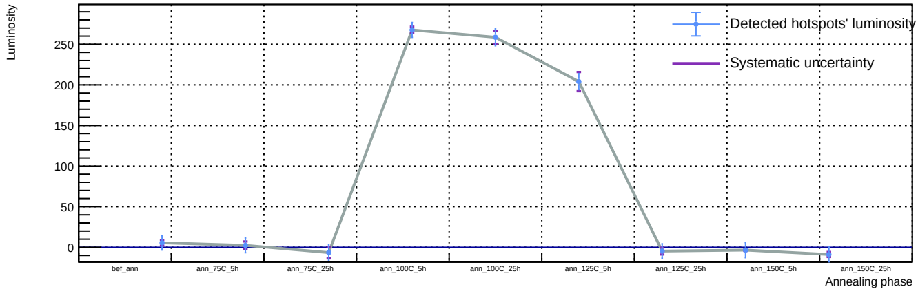
Sensor A1, T = 20\text{ C} , v_{\text{over}} = 7\text{ V} - Spot 78: luminosity vs phase
