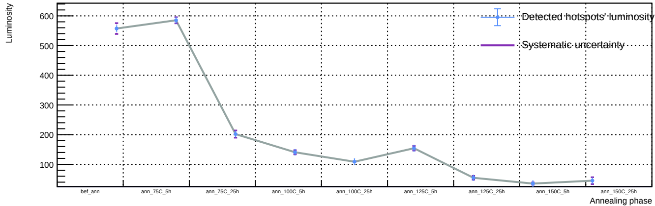
Sensor A1, T = 20\text{ C} , v_{\text{over}} = 7\text{ V} - Spot 8: luminosity vs phase
