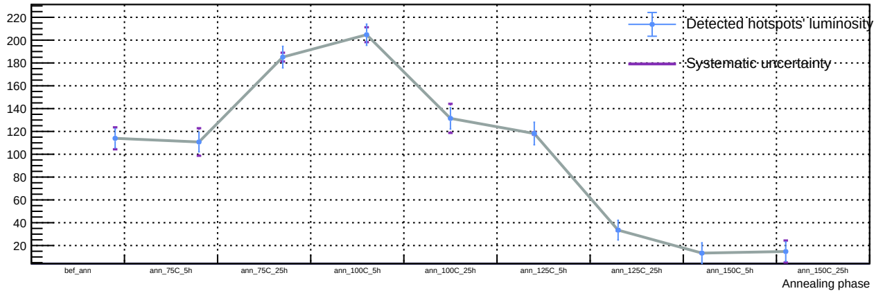
Sensor A1, T = 20\text{ C} , v_{\text{over}} = 7\text{ V} - Spot 82: luminosity vs phase
