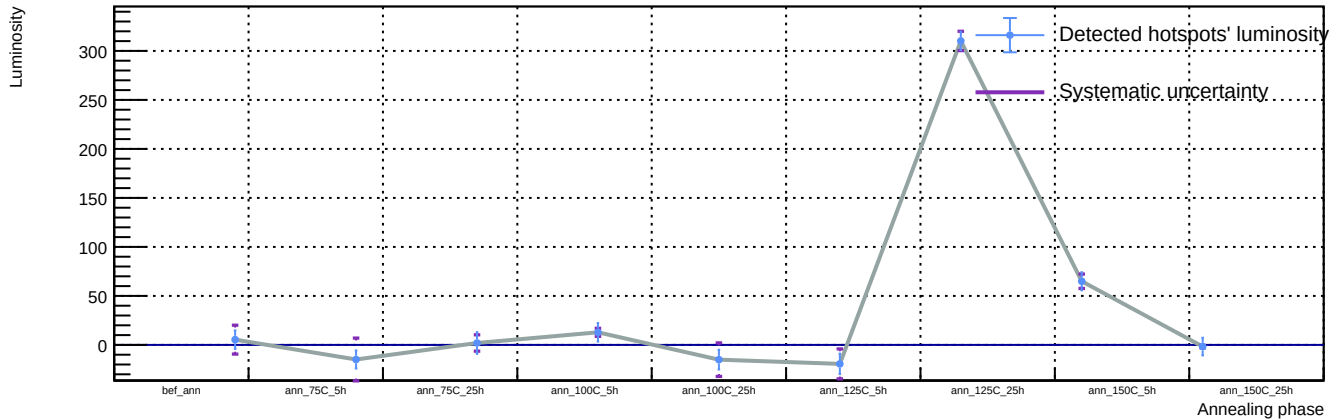
Sensor A1, T = 20\text{ C} , v_{\text{over}} = 7\text{ V} - Spot 83: luminosity vs phase
