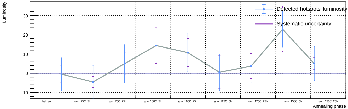
Sensor A1, T = 20\text{ C} , v_{\text{over}} = 7\text{ V} - Spot 89: luminosity vs phase
