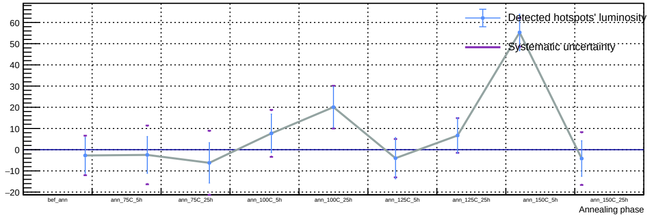
Sensor A1, T = 20\text{ C} , v_{\text{over}} = 7\text{ V} - Spot 90: luminosity vs phase
