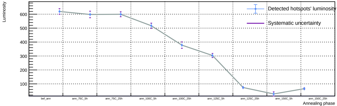
Sensor A1, T = 20\text{ C} , v_{\text{over}} = 7\text{ V} - Spot 95: luminosity vs phase
