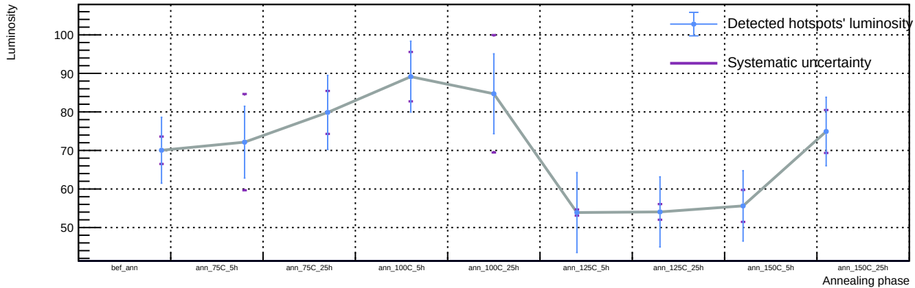
Sensor A1, T = 20\text{ C} , v_{\text{over}} = 7\text{ V} - Spot 96: luminosity vs phase
