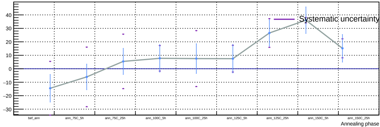
Sensor A1, T = 20\text{ C} , v_{\text{over}} = 7\text{ V} - Spot 97: luminosity vs phase
