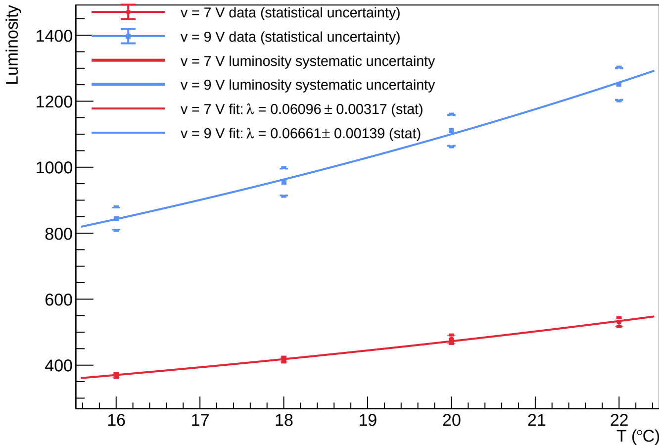
A1 - Spot 0: luminosity vs temperature at v = 7 V and v = 9 V
