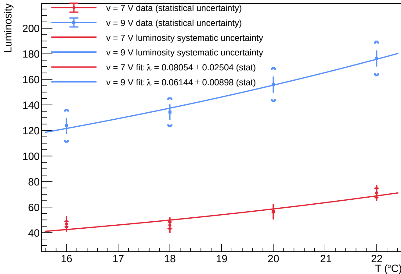
A1 - Spot 10: luminosity vs temperature at v = 7 V and v = 9 V
