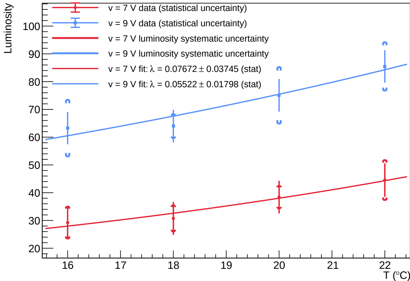
A1 - Spot 2: luminosity vs temperature at v = 7 V and v = 9 V
