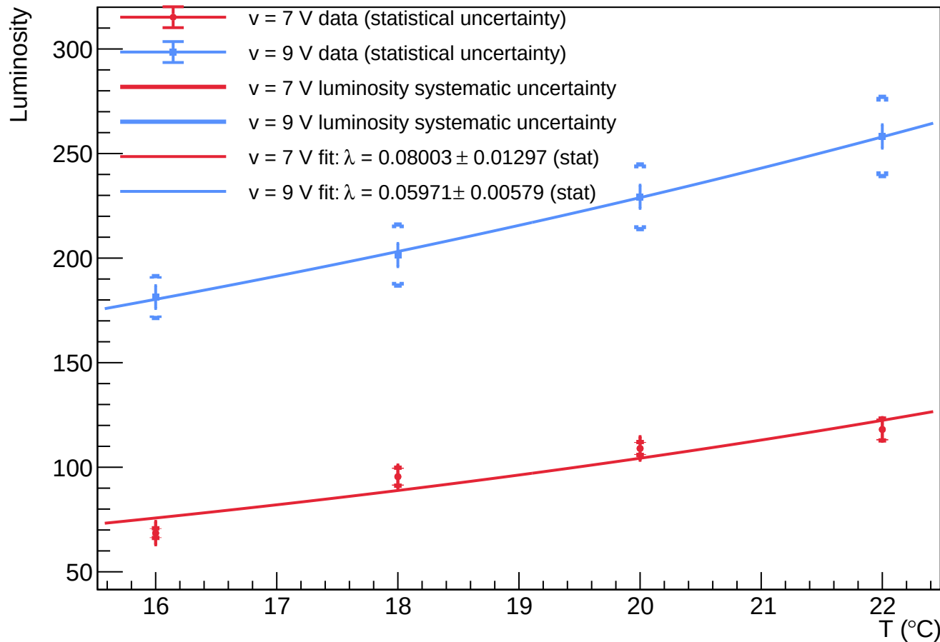
A1 - Spot 3: luminosity vs temperature at v = 7 V and v = 9 V
