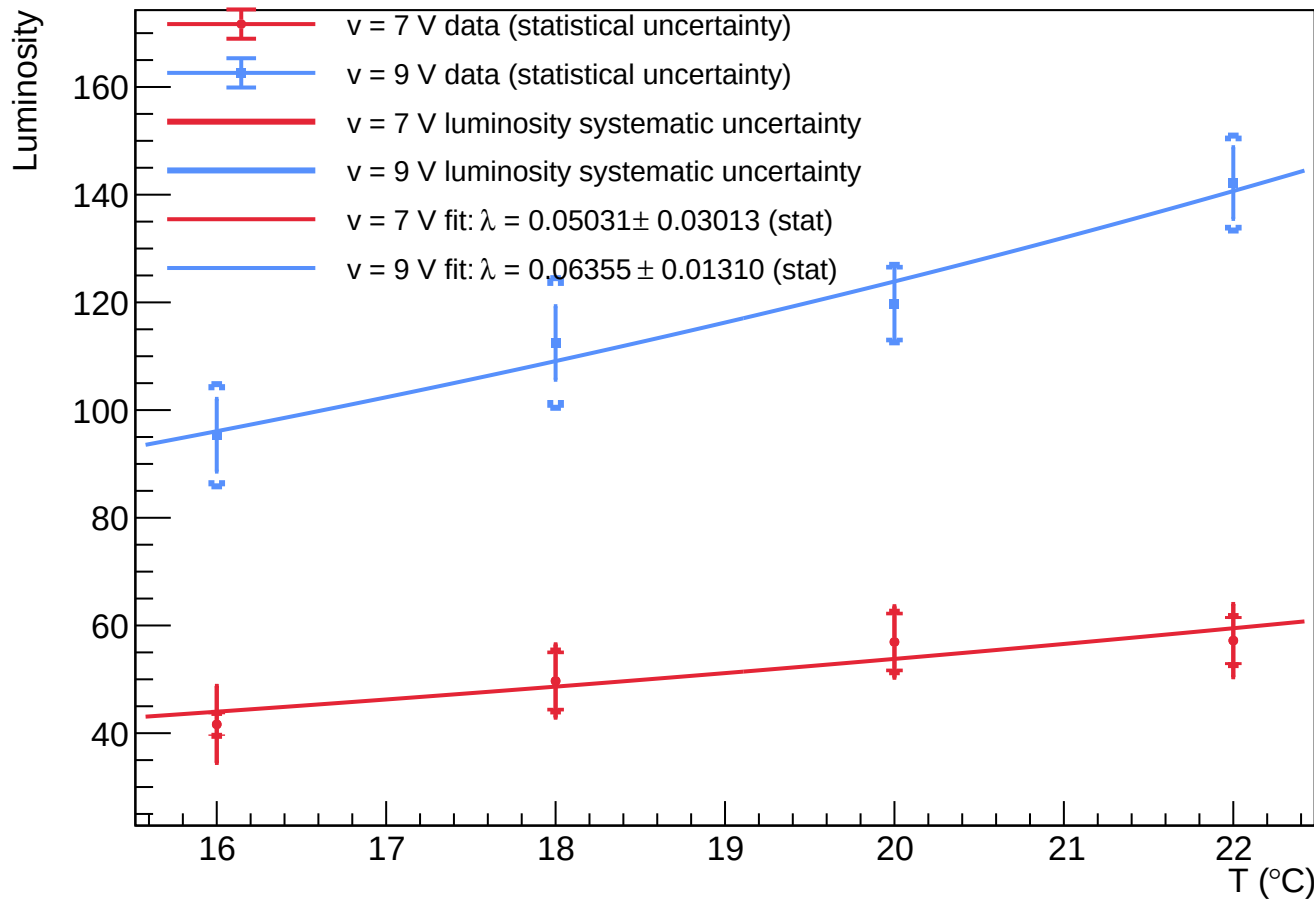
A1 - Spot 4: luminosity vs temperature at v = 7 V and v = 9 V
