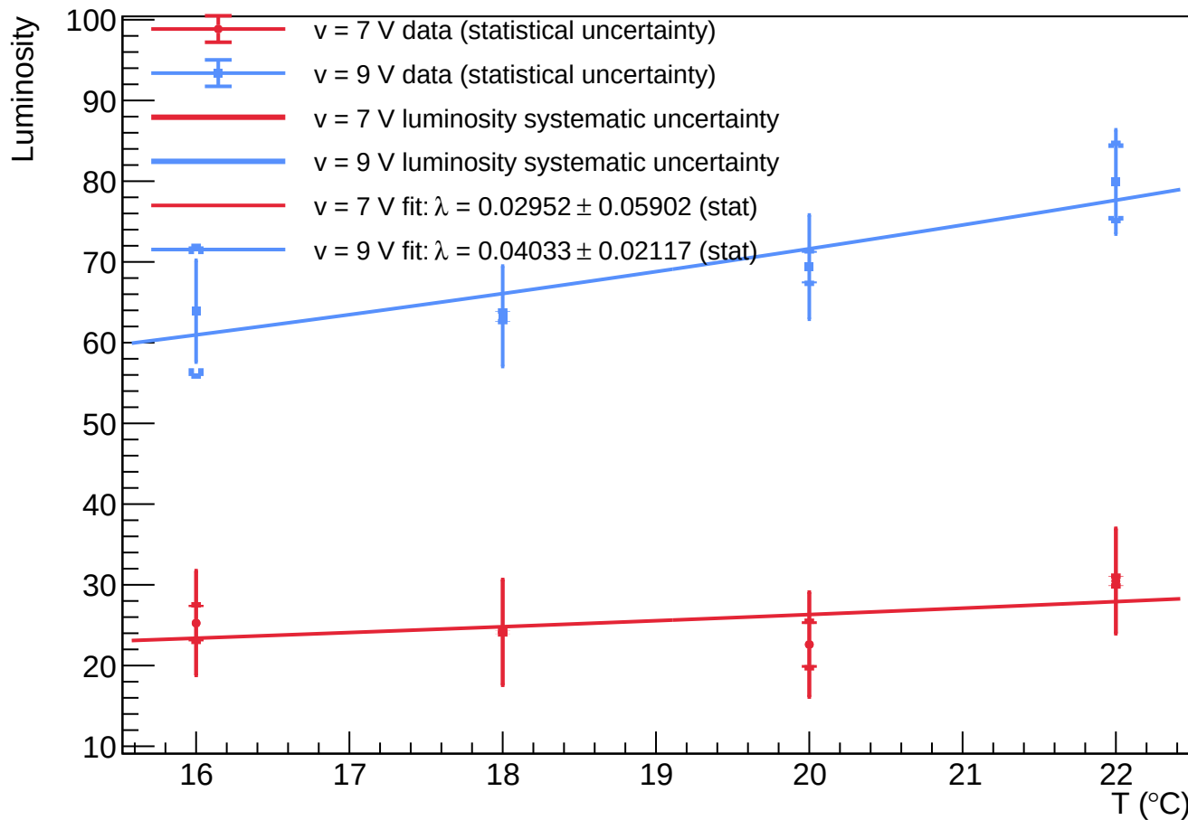
A1 - Spot 5: luminosity vs temperature at v = 7 V and v = 9 V
