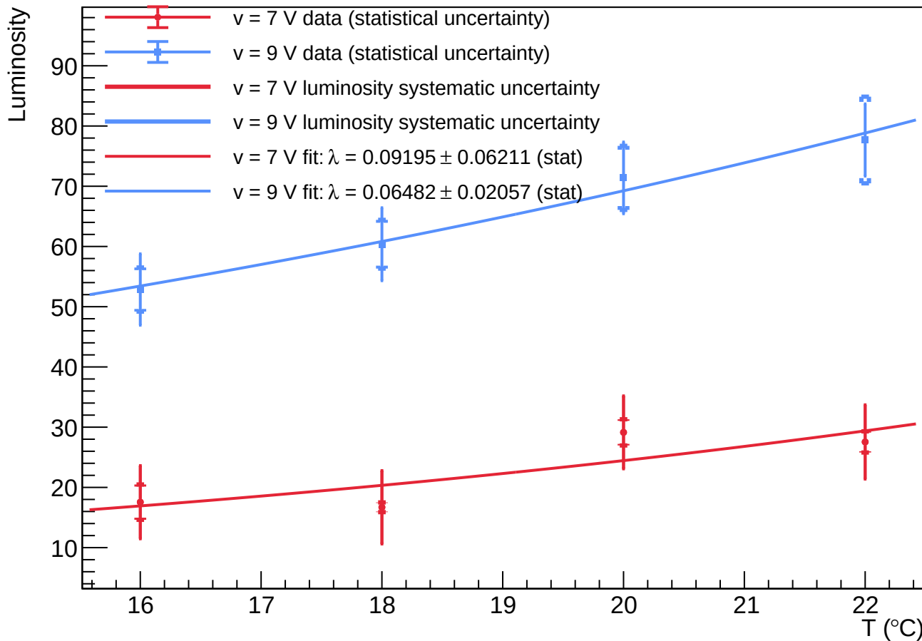
A1 - Spot 6: luminosity vs temperature at v = 7 V and v = 9 V
