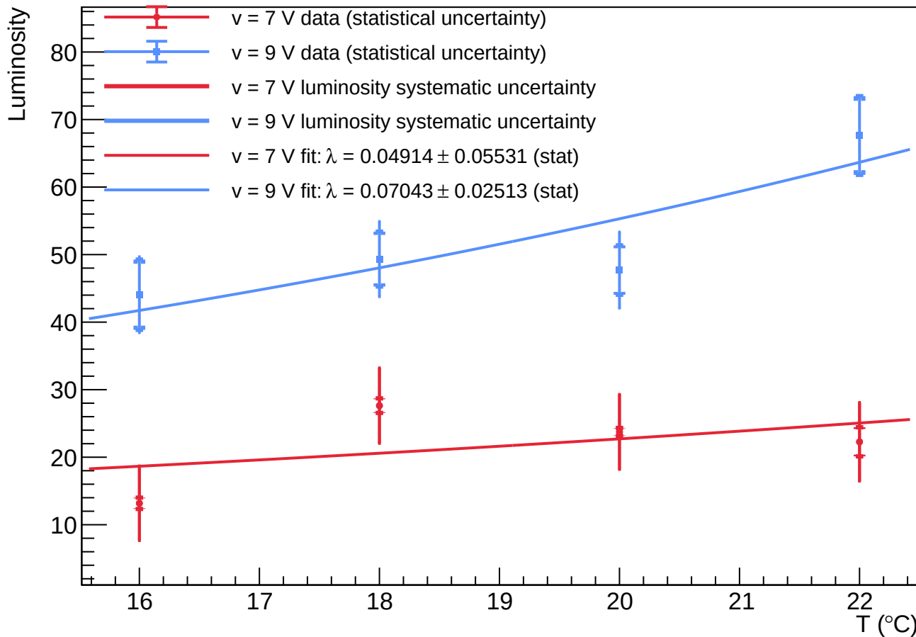
A1 - Spot 7: luminosity vs temperature at v = 7 V and v = 9 V
