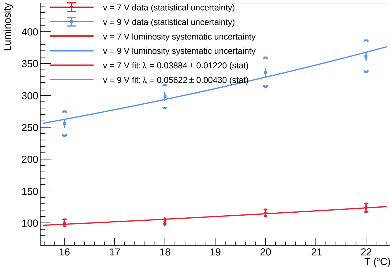
A1 - Spot 8: luminosity vs temperature at v = 7 V and v = 9 V
