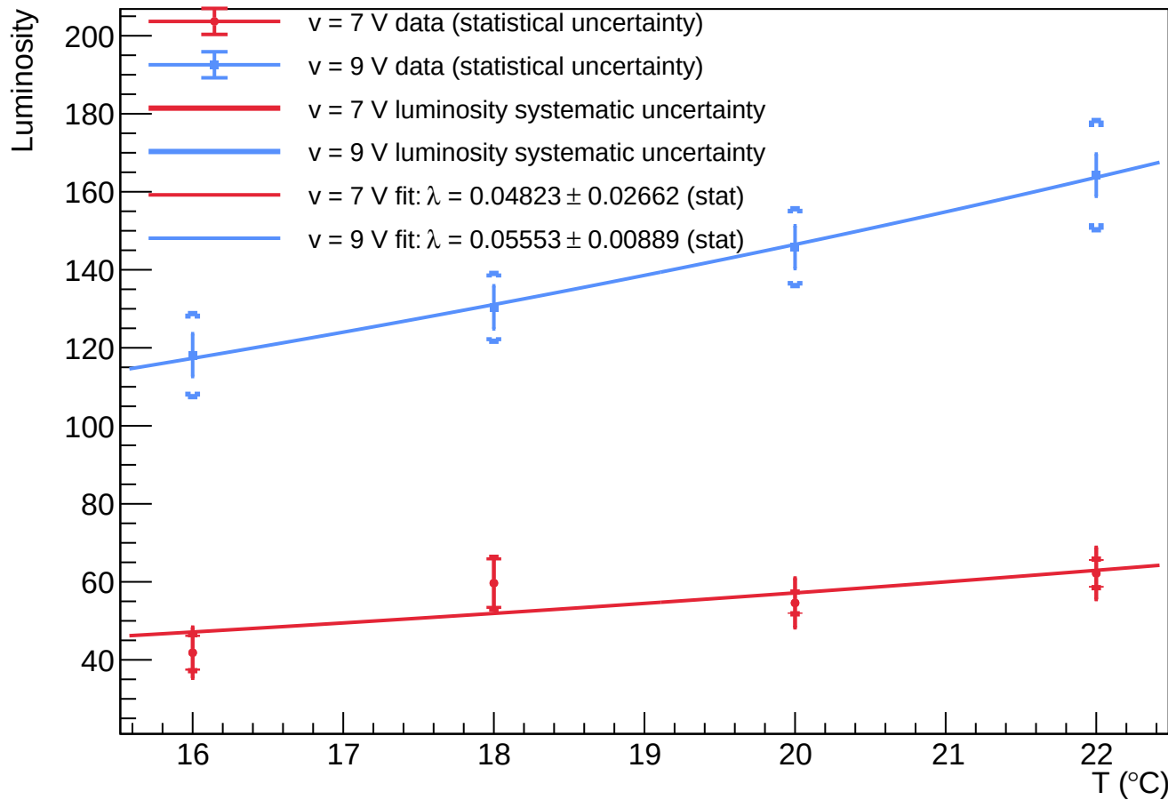
A1 - Spot 9: luminosity vs temperature at \nu = 7 V and \nu = 9 V
