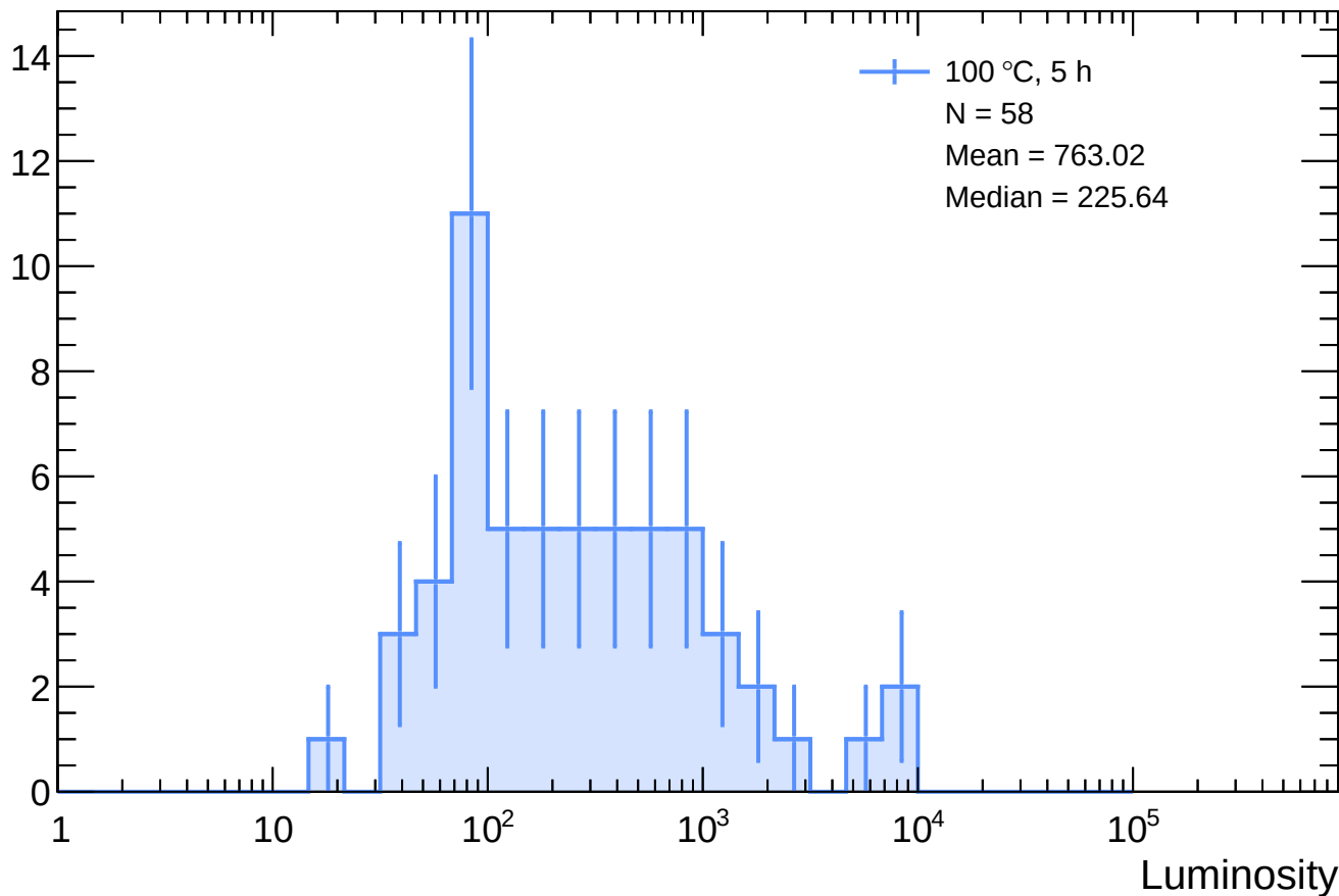
Sensor A1 - 100 °C, 5 h luminosity distribution
