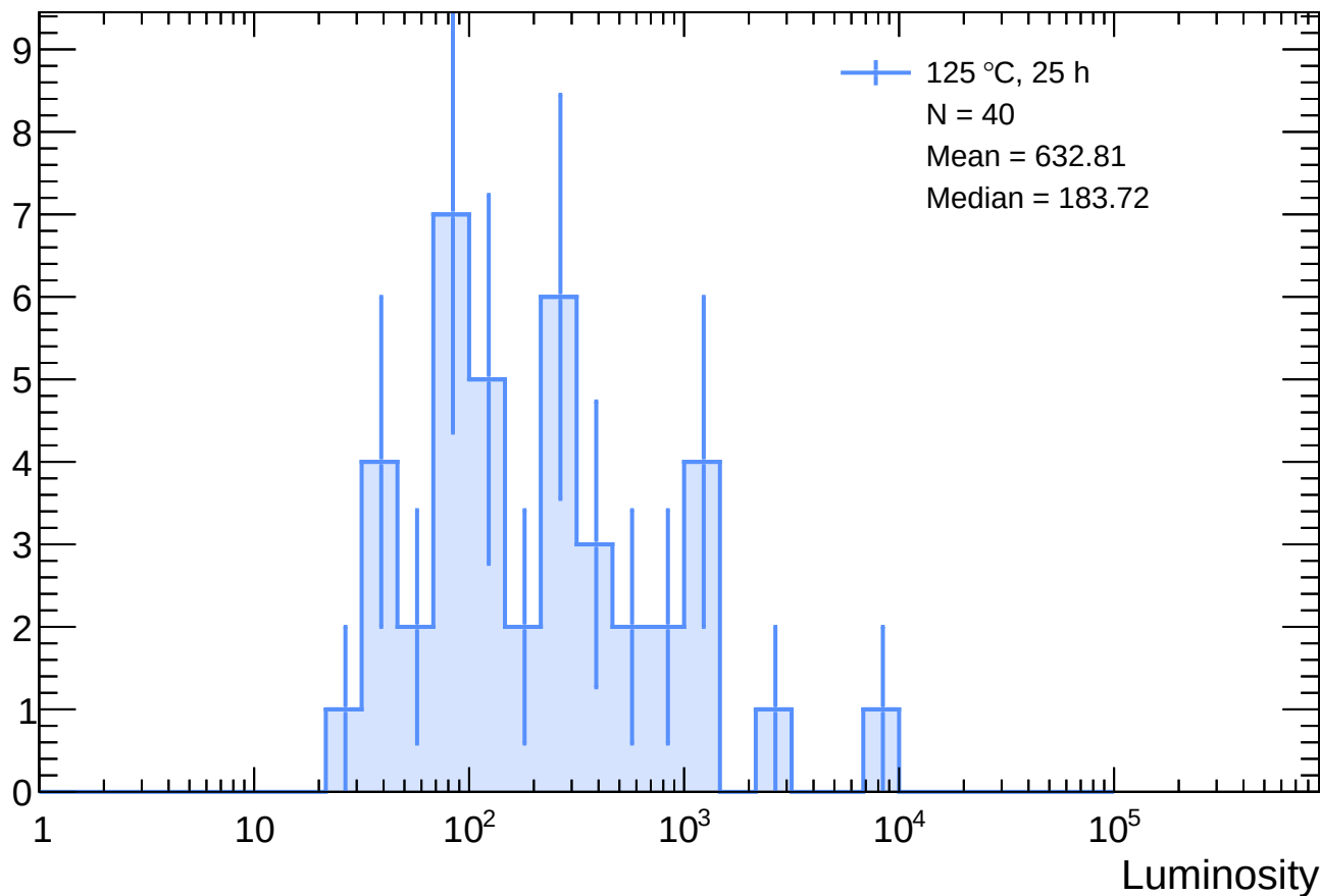
Sensor A1 - 125 °C, 25 h luminosity distribution
