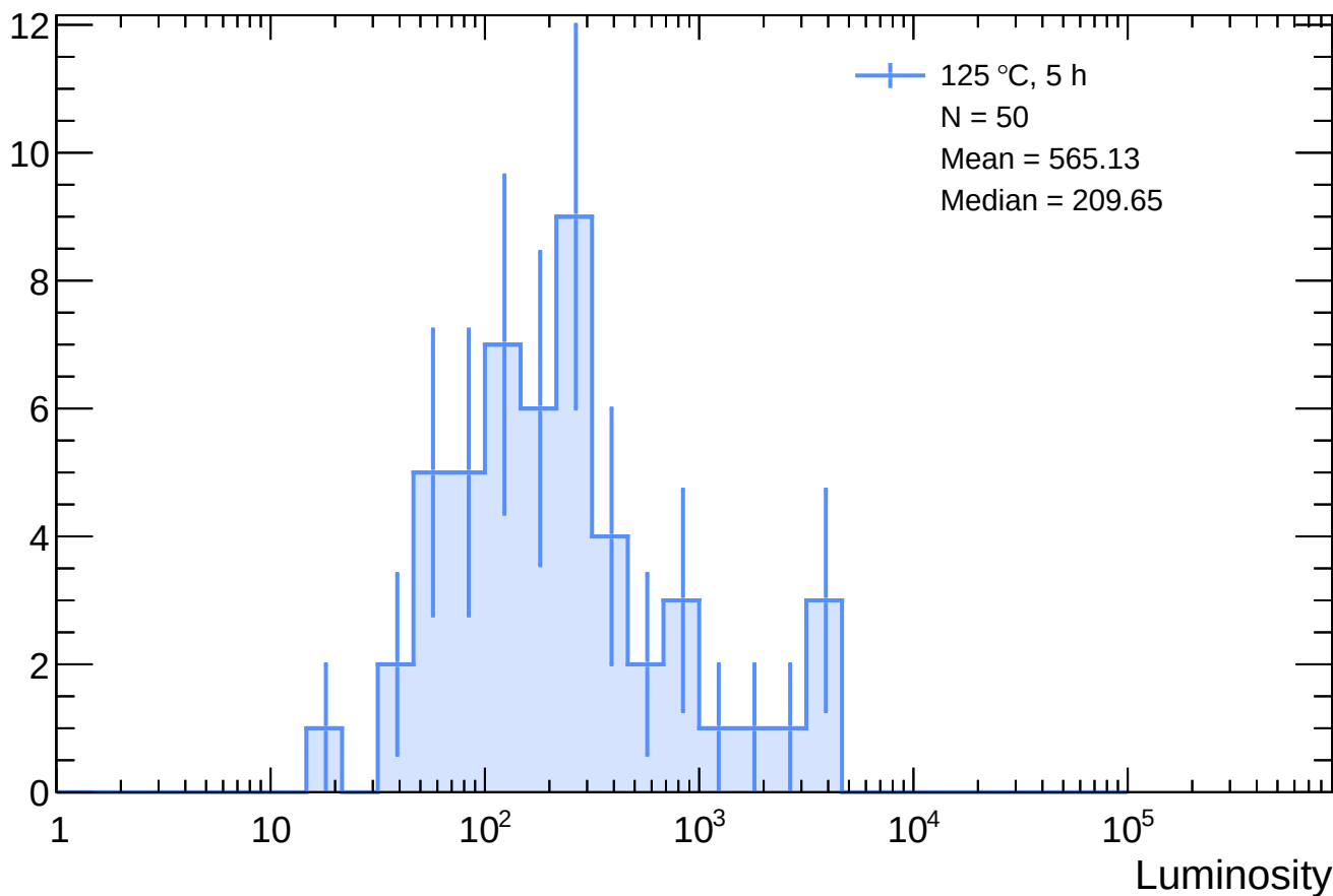
Sensor A1 - 125 °C, 5 h luminosity distribution
