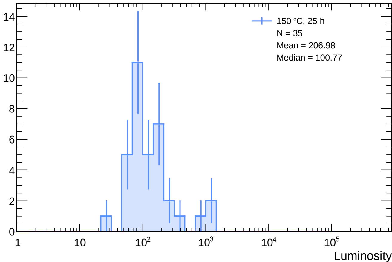
Sensor A1 - 150 °C, 25 h luminosity distribution
