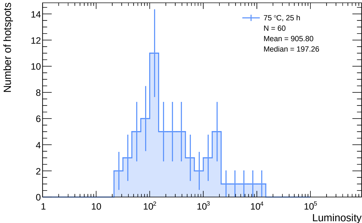
Sensor A1 - 75 °C, 25 h luminosity distribution
