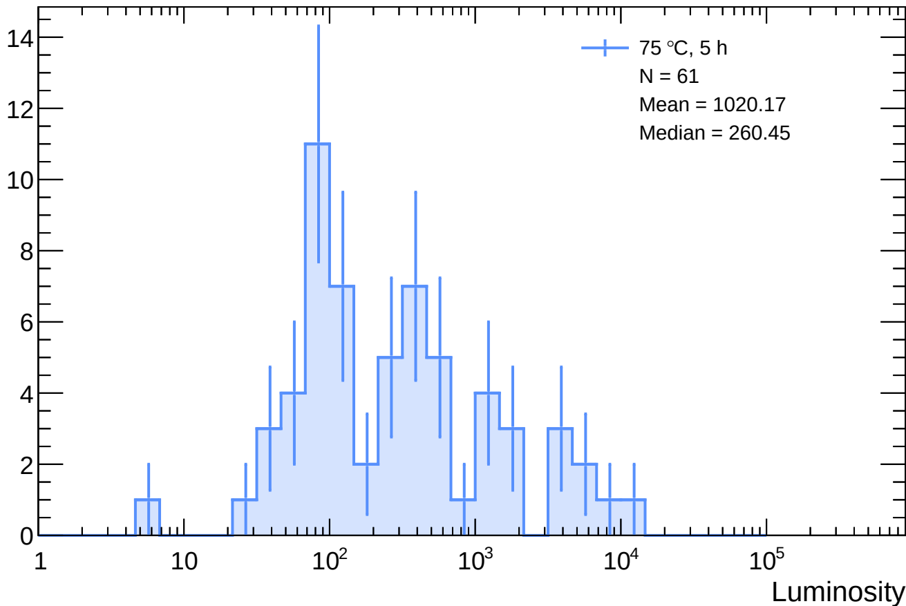
Sensor A1 - 75 °C, 5 h luminosity distribution
