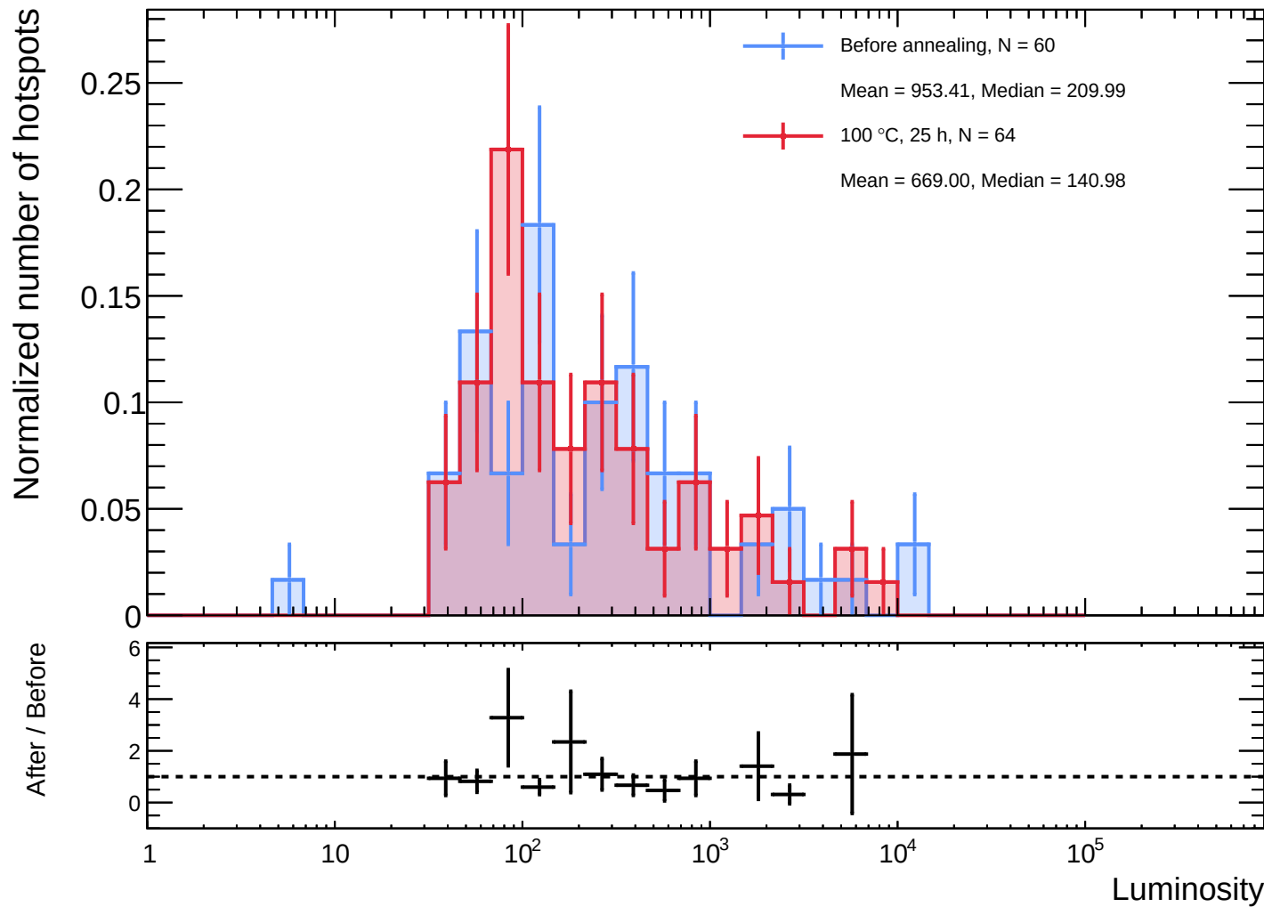
Sensor A1 - Before annealing vs 100 °C, 25 h luminosity distributions
