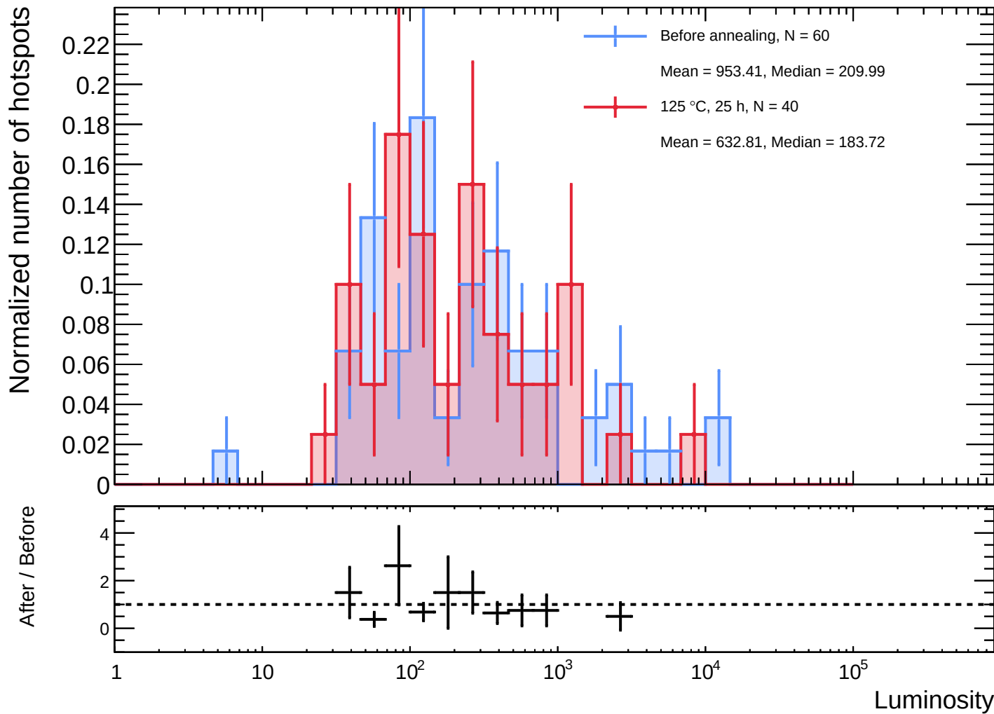
Sensor A1 - Before annealing vs 125 °C, 25 h luminosity distributions
