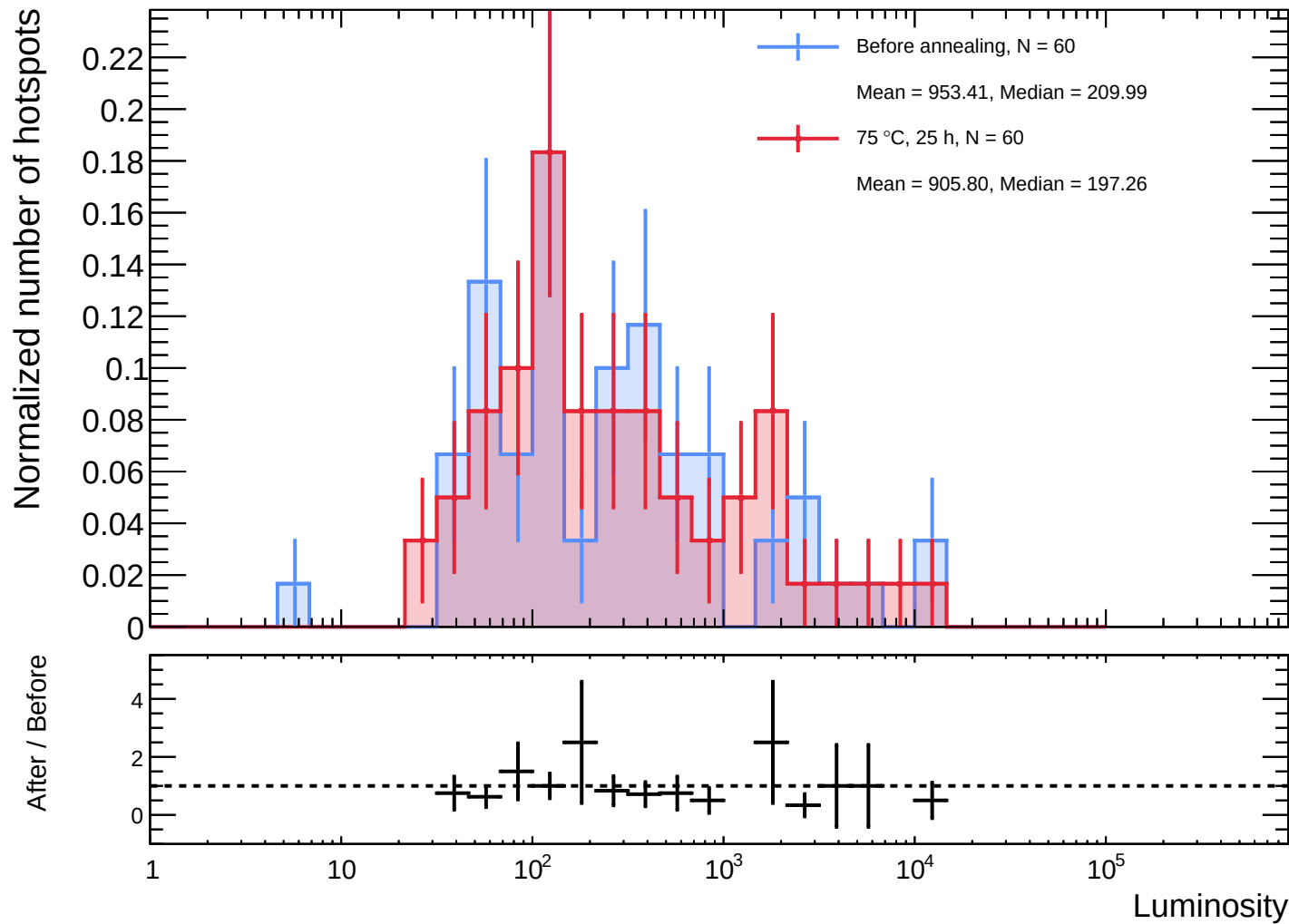
Sensor A1 - Before annealing vs 75 °C, 25 h luminosity distributions
