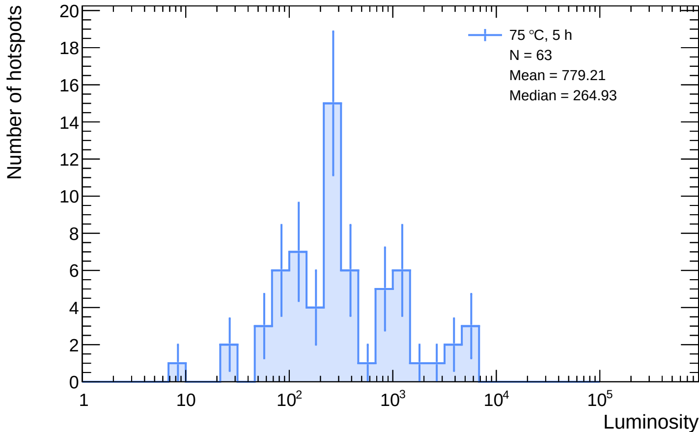
Sensor B1 - 75 °C, 5 h luminosity distribution
