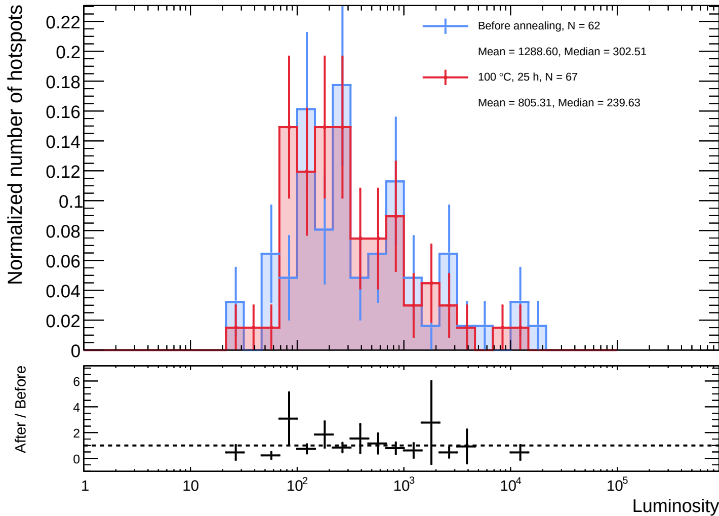
Sensor B1 - Before annealing vs 100 °C, 25 h luminosity distributions
