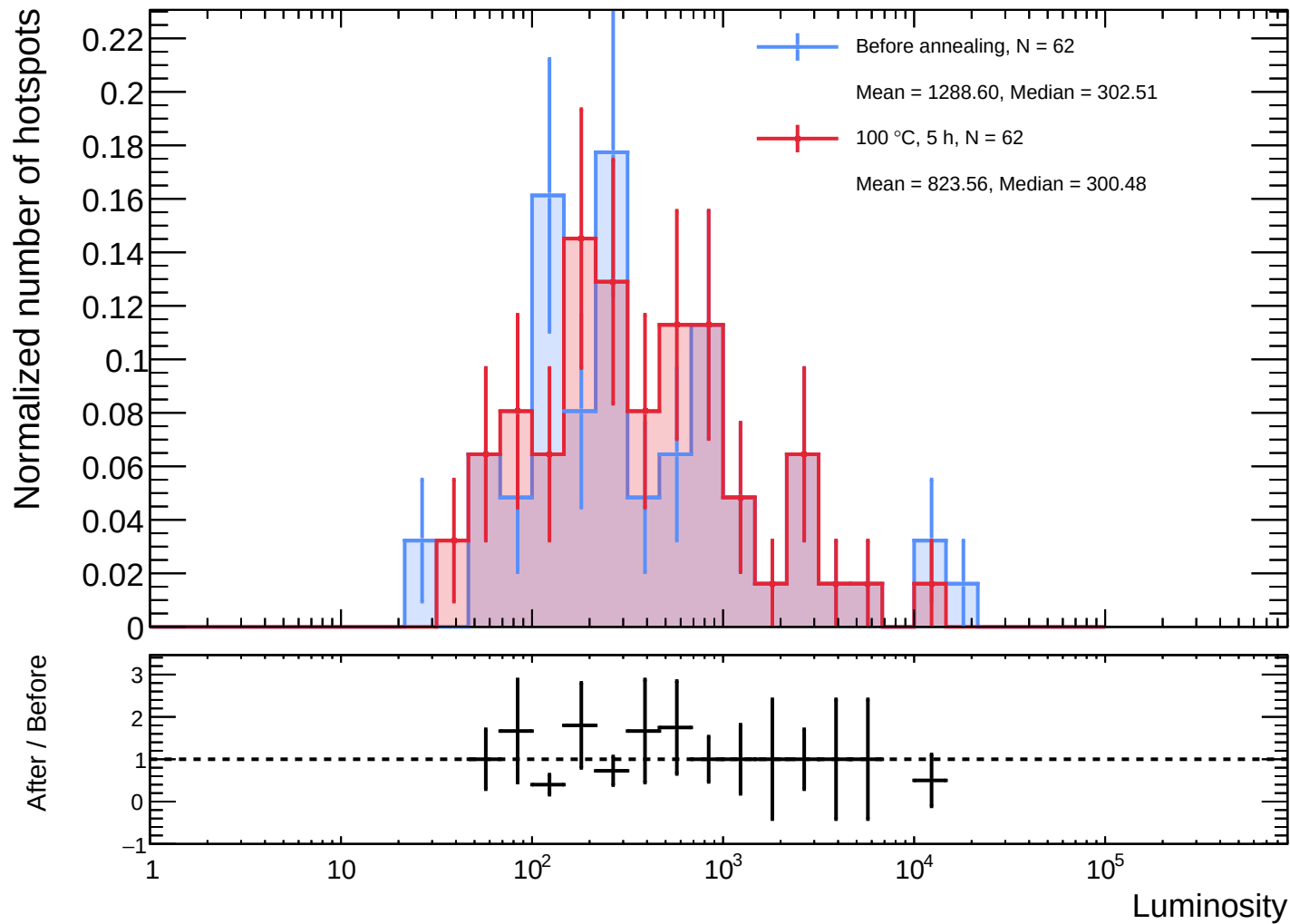
Sensor B1 - Before annealing vs 100 °C, 5 h luminosity distributions
