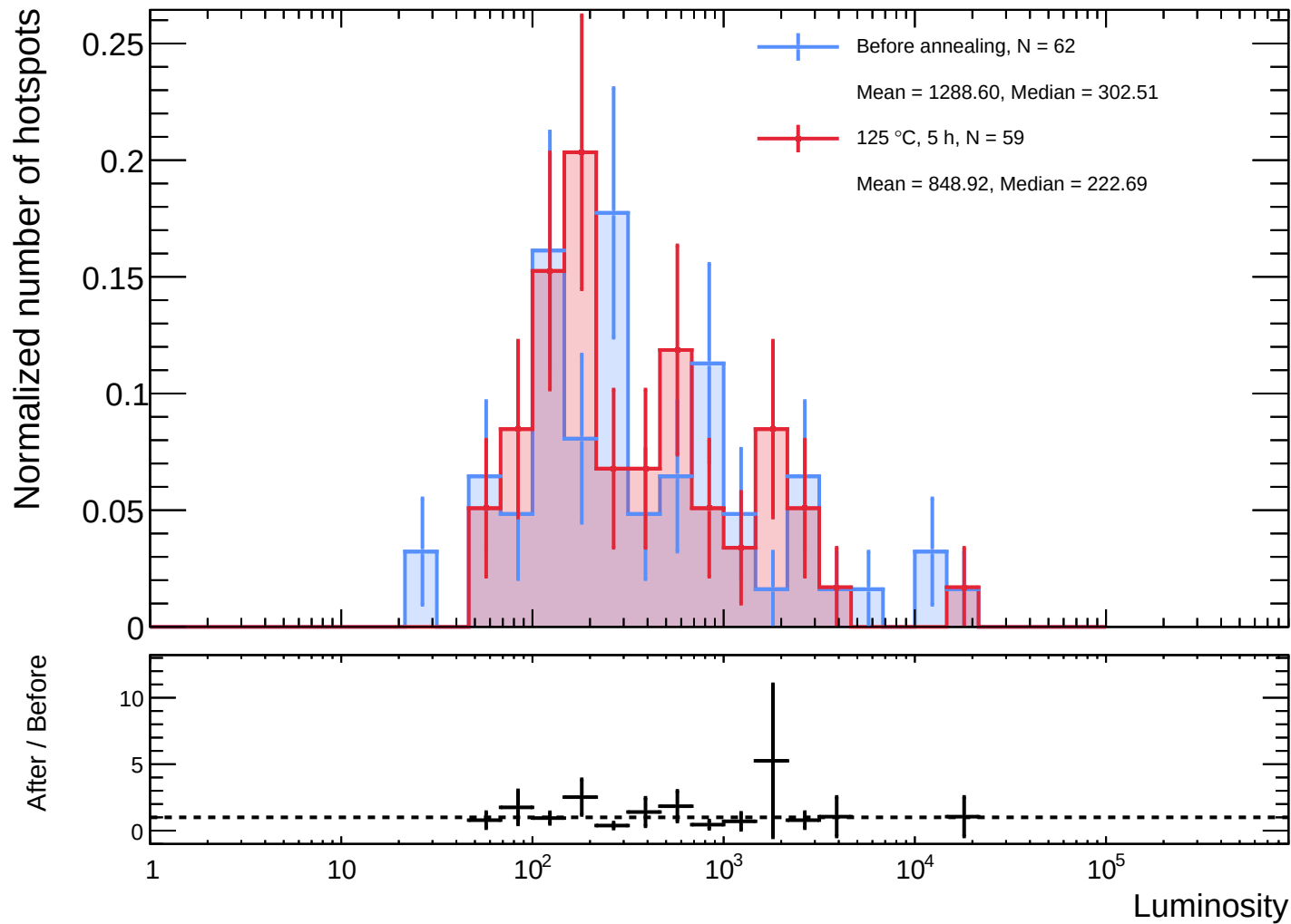
Sensor B1 - Before annealing vs 125 °C, 5 h luminosity distributions
