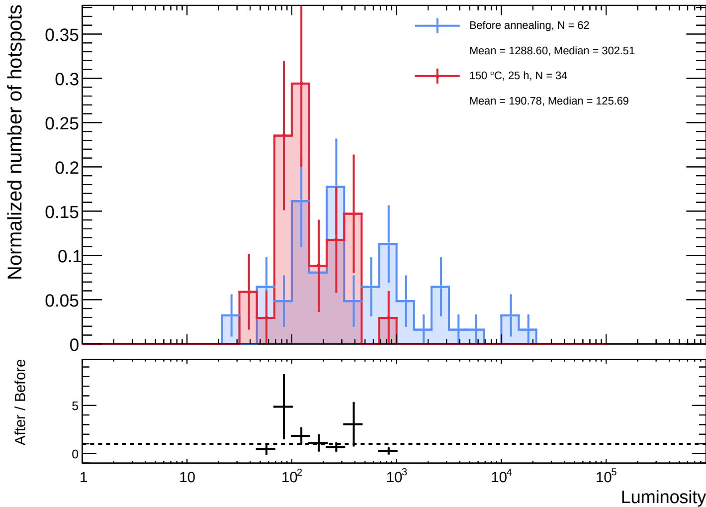
Sensor B1 - Before annealing vs 150 °C, 25 h luminosity distributions
