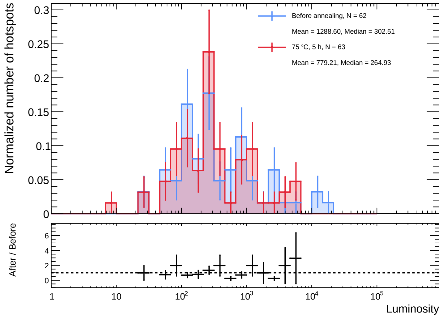
Sensor B1 - Before annealing vs 75 °C, 5 h luminosity distributions
