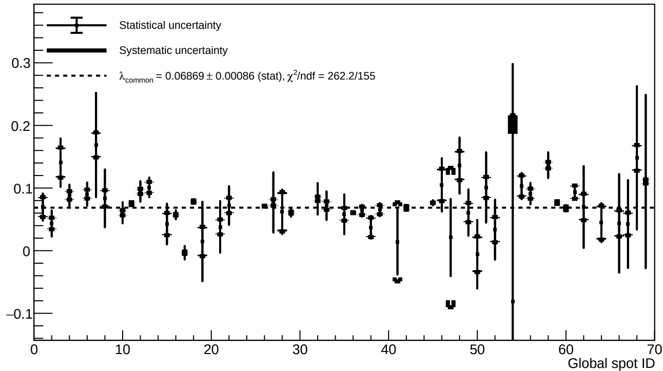
B1_v=3_before_annealing - Exponential fit parameter \lambda - before_annealing
