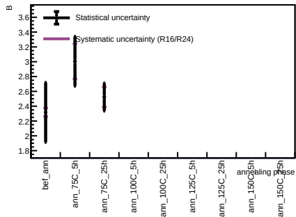
Sensor A1, T = 20 C - Spot 9
