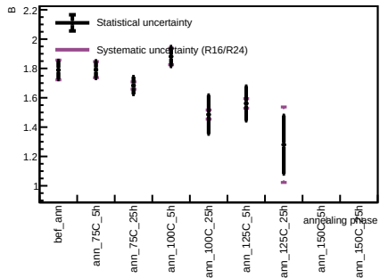
Sensor A1, T = 20 C - Spot 10
