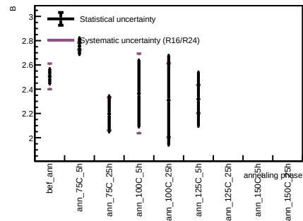
Sensor A1, T = 20 C - Spot 8
