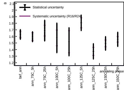
Sensor A1, T = 20 C - Spot 17
