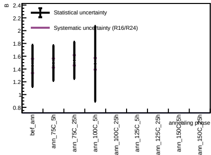
Sensor A1, T = 20 C - Spot 16
