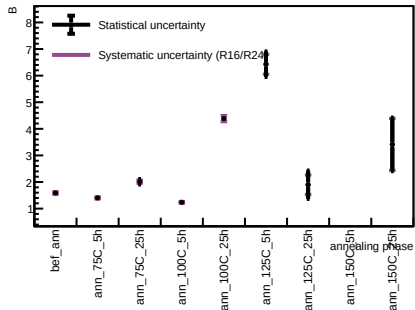
Sensor A1, T = 20 C - Spot 37
