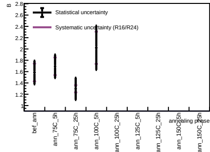
Sensor A1, T = 20 C - Spot 41
