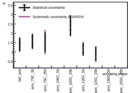
Sensor A1, T = 20 C - Spot 40
