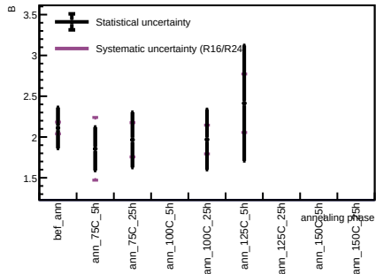
Sensor A1, T = 20 C - Spot 36
