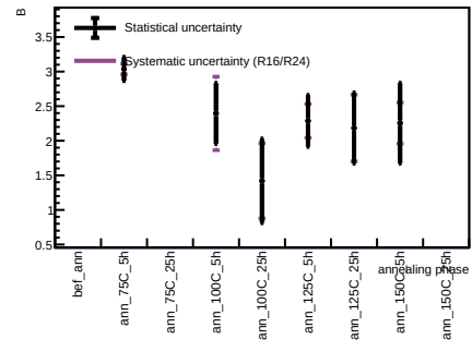
Sensor A1, T = 20 C - Spot 65
