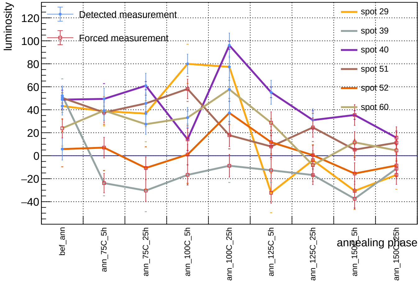
Sensor A1, T = 20 C, representative v = 58.3 V (max available) - luminosity vs phase - order 10 1
