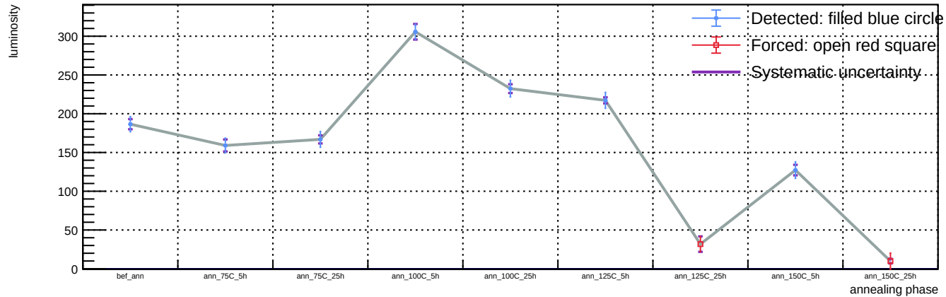
Sensor A1, T = 20 C, representative v = 58.3 V (max available) - Spot 1: luminosity vs phase
