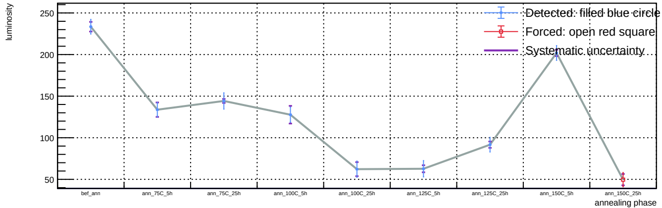
Sensor A1, T = 20 C, representative v = 58.3 V (max available) - Spot 19: luminosity vs phase
