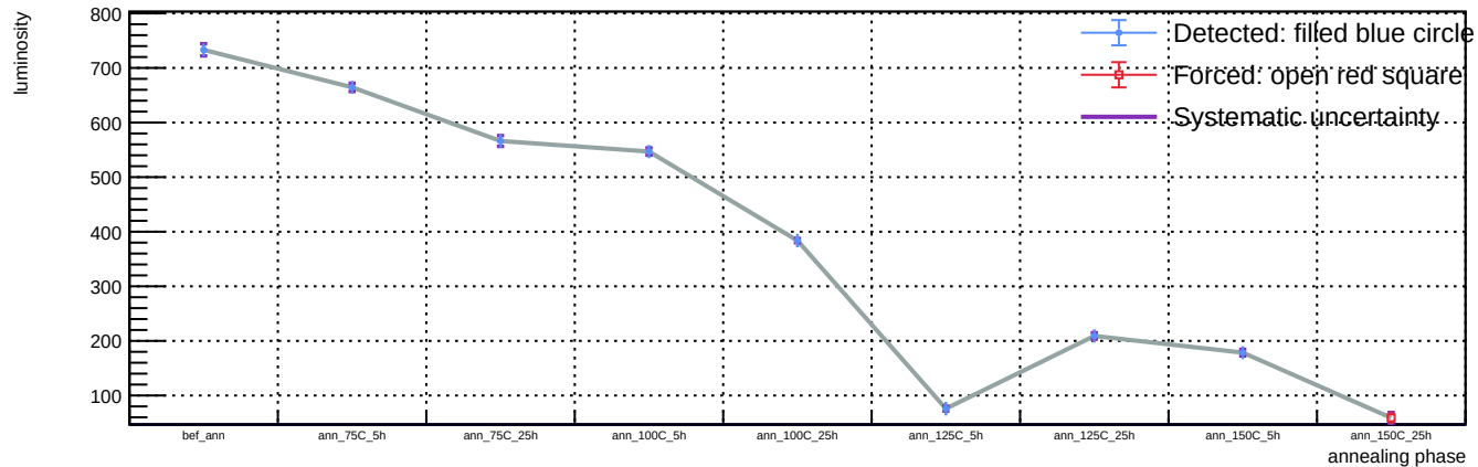
Sensor A1, T = 20 C, representative v = 58.3 V (max available) - Spot 4: luminosity vs phase
