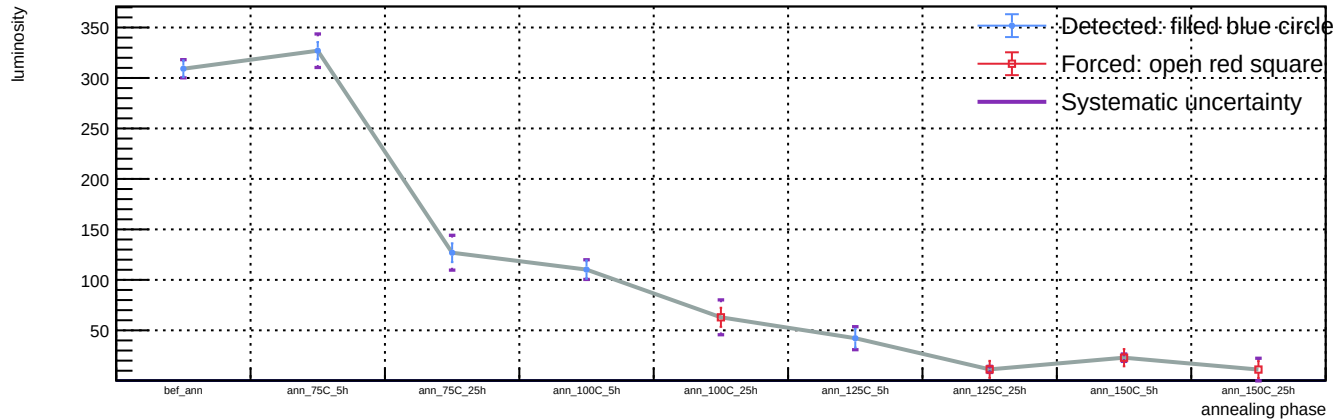
Sensor A1, T = 20 C, representative v = 58.3 V (max available) - Spot 49: luminosity vs phase
