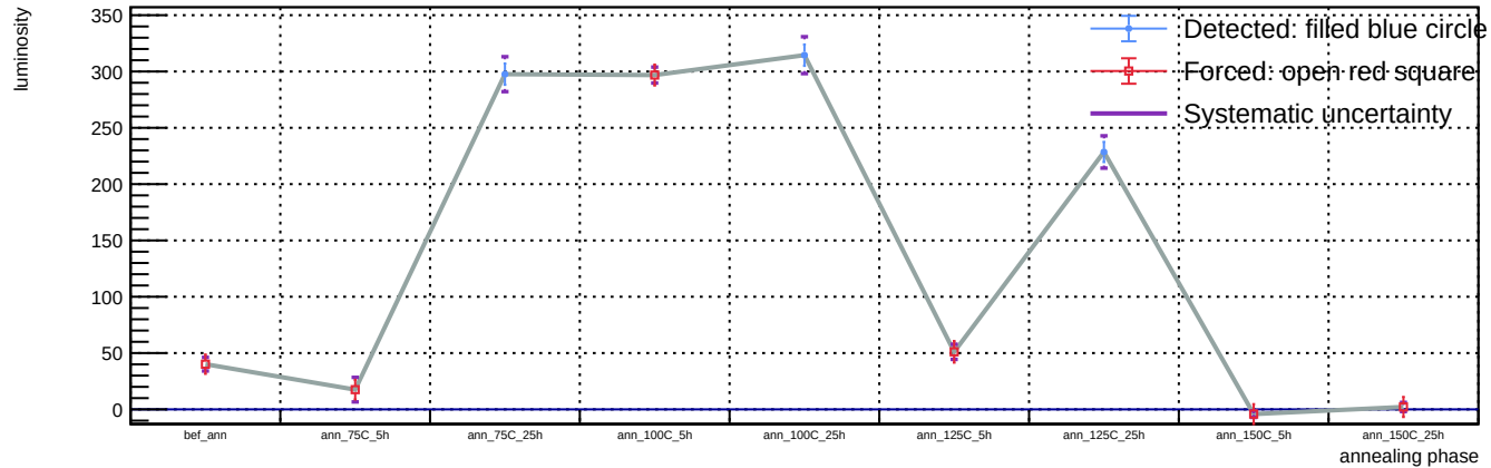
Sensor A1, T = 20 C, representative v = 58.3 V (max available) - Spot 66: luminosity vs phase
