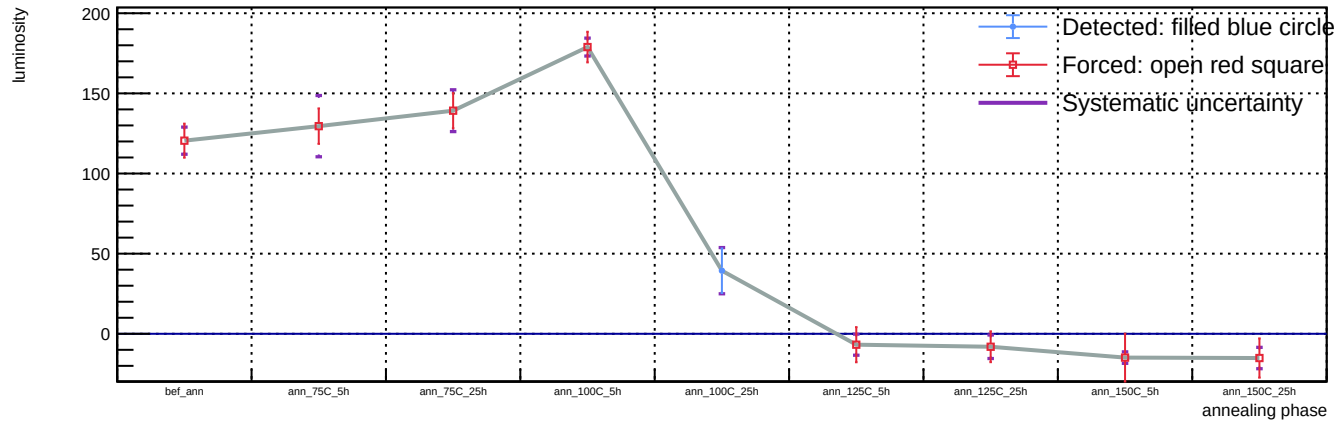
Sensor A1, T = 20 C, representative v = 58.3 V (max available) - Spot 74: luminosity vs phase
