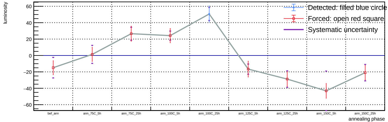
Sensor A1, T = 20 C, representative v = 58.3 V (max available) - Spot 76: luminosity vs phase
