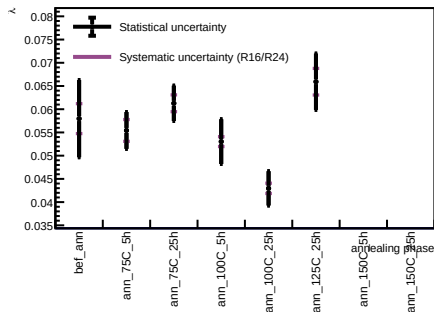
Sensor A1, v = 5 V - Spot 7
