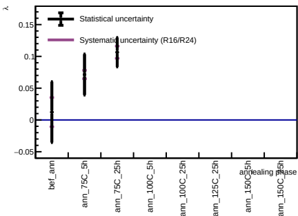
Sensor A1, v = 5 V - Spot 9
