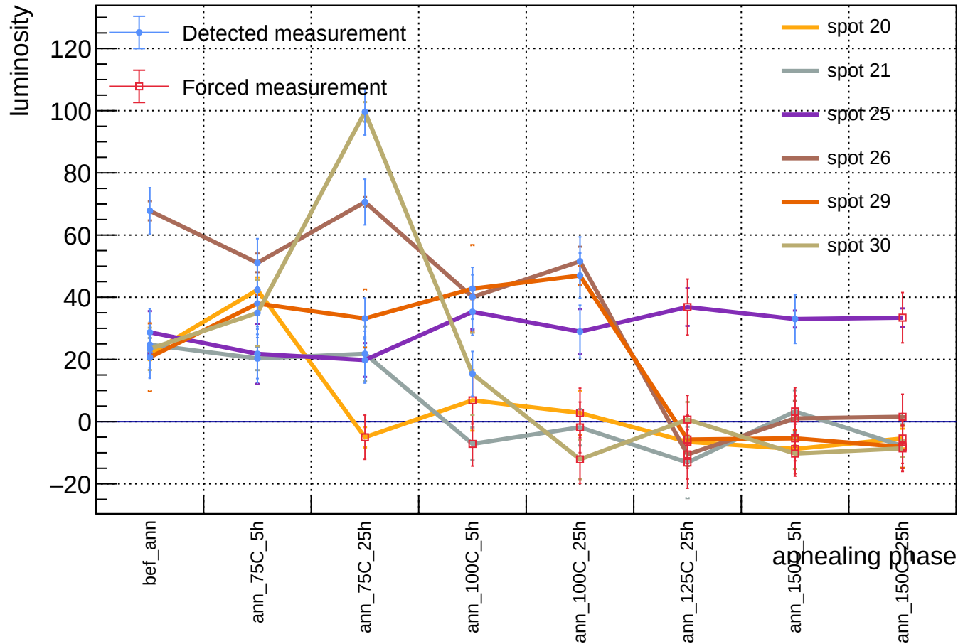
Sensor A1, v = 5 V, representative T = 23 C (max available) - luminosity vs phase - order 10^1
